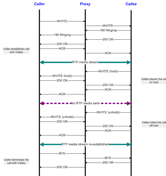
Figure 6-8. Call Hold
