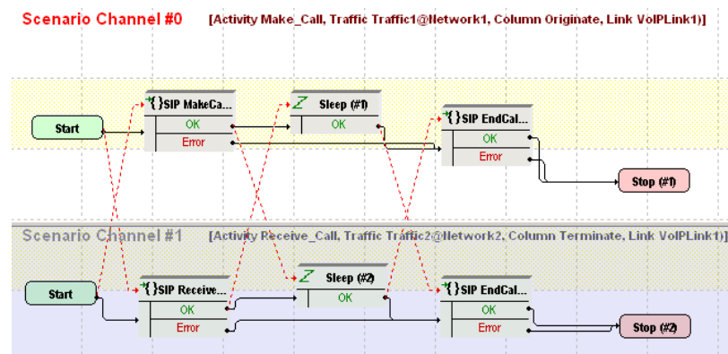
Figure 5-26. SC_001_B2B_SIPv4_T1_BasicCall
