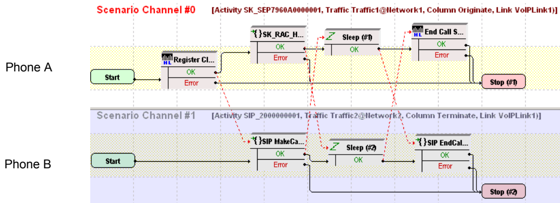
Figure 5-70. MIX_008_7960_SO_US_80k_BHCA_IPv4_Static_SIP_to_SK_trunk_Bulk_Call Test Scenario
