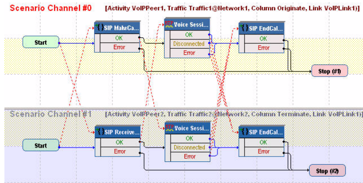
Figure 5-2. VS_004_B2B_SIPv4 MakeCall - ReceiveCall - EndCall - Early Media
