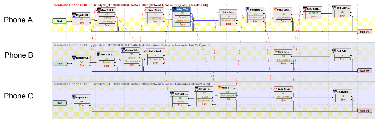
Figure 5-48. SK_031_7960_SM_US_5_ChS_IPv4_Static_List_Ad_Hoc_Conference Test Scenario
