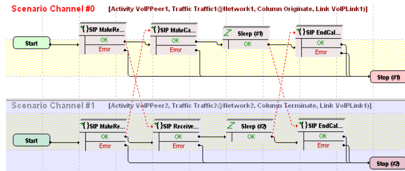
Figure 4-5. VS_007_DUT_SIPv4 Make-Receive Call with ReRegistration Test Scenario
