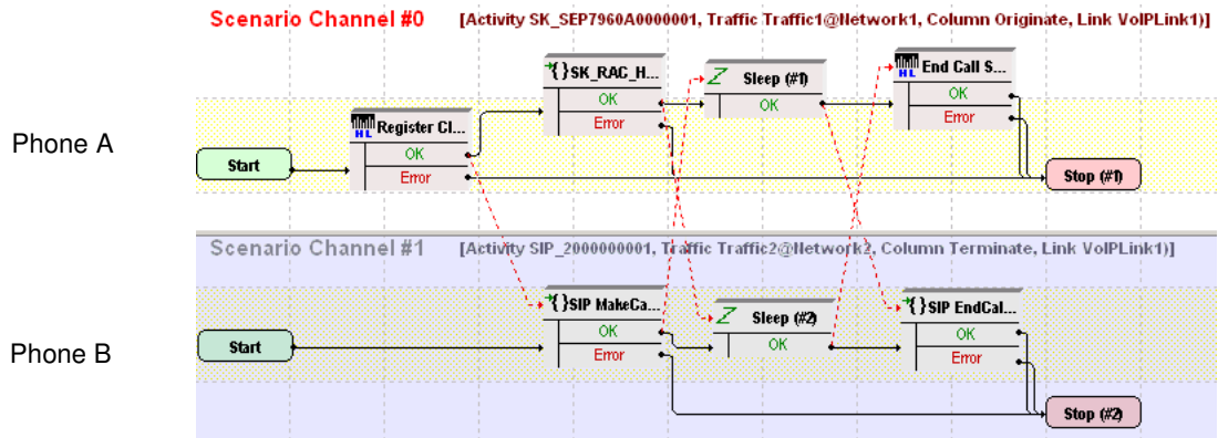
Figure 4-76. MIX_008_7960_SO_US_80k_BHCA_IPv4_Static_SIP_to_SK_trunk_Bulk_Call Test Scenario
