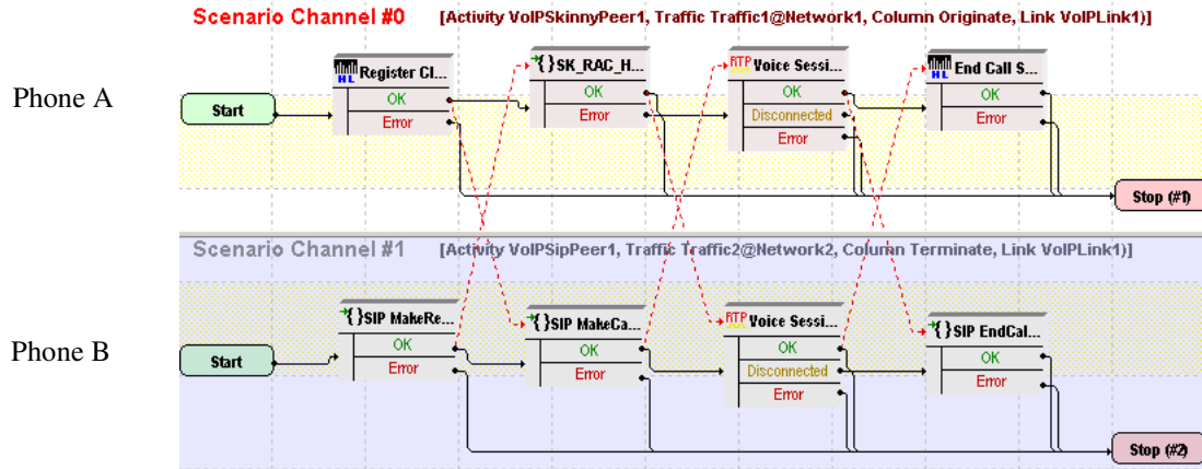
Figure 4-68. MIX_020_7960_SM_US_900_Channels_IPv4_Static_SIP_to_Skinny_Call_Voice_10s Test Scenario
