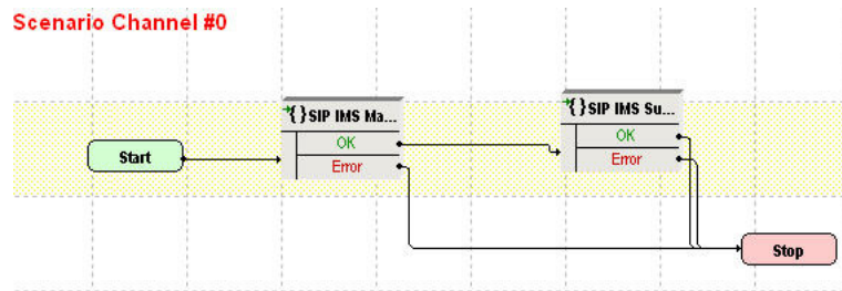
Figure 4-13. VS_018_DUT_SIPv4 IMS Registration with Subscription
