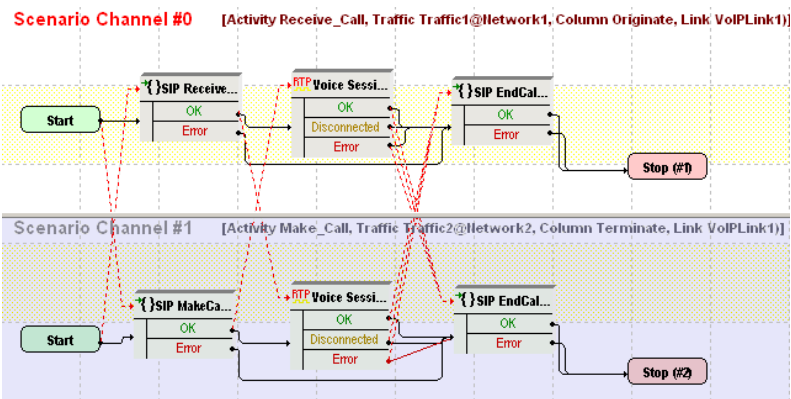
Figure 4-37. SC_013_B2B_SIPv4_T2_BasicCall_between_two_Clouds_RTP_n_to_n
