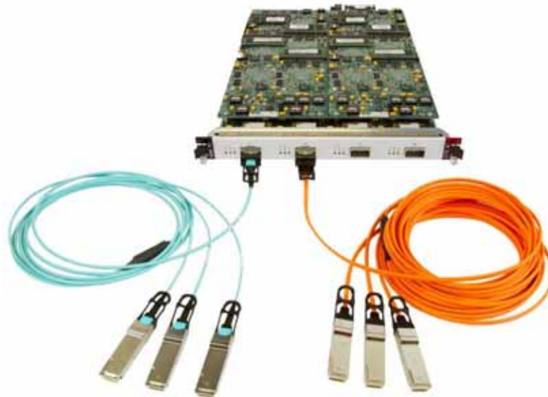
Figure 34-21. Xcellon-Multis load module with CXP-to-3x40GE fan-out
