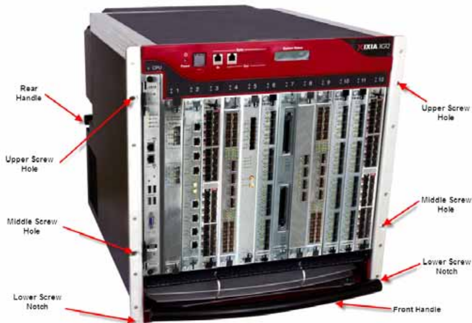
Figure 6-2. Safety Features
