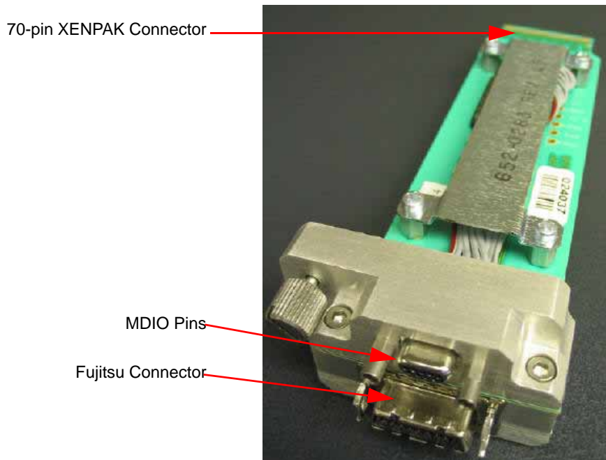
Figure 24-14. XAUI Fujitsu to XENPAK Adapter
