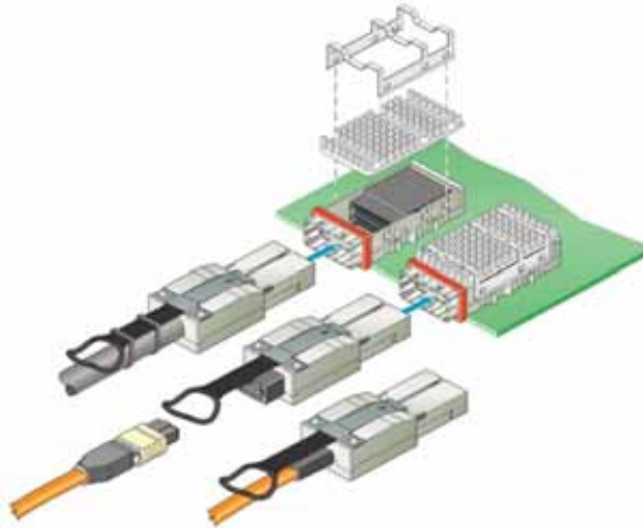
Figure 34-24. CXP Active Copper, Optical (pluggable), Active Optical
