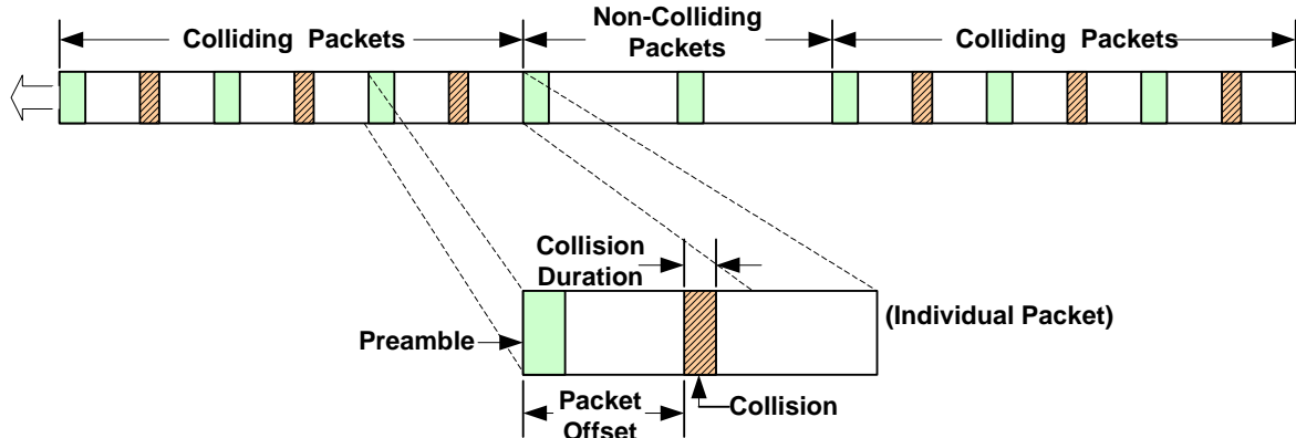
Figure 2-50. Forced Collisions
