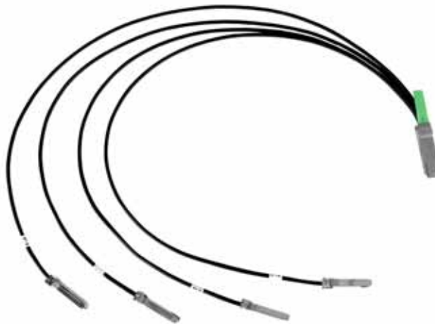
Figure 34-19. QSFP-to-4x10GE SFP+ Direct Attach Cable (DAC) cable
