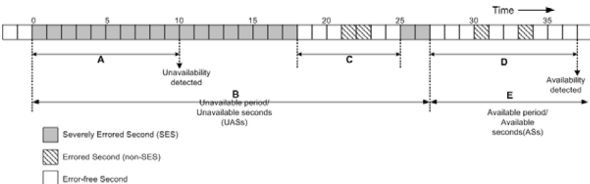
Figure 2-35. BERT—Unavailable/Available Periods
