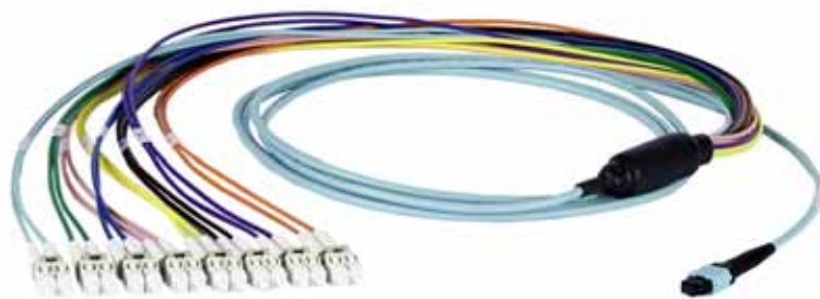
Figure 34-18.MT-MT 8x10GE passive fiber fan-out cable
