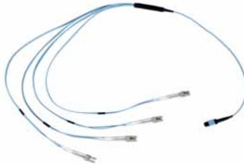
Figure 34-17.MT-MT 4x10GE passive fiber fan-out cable
