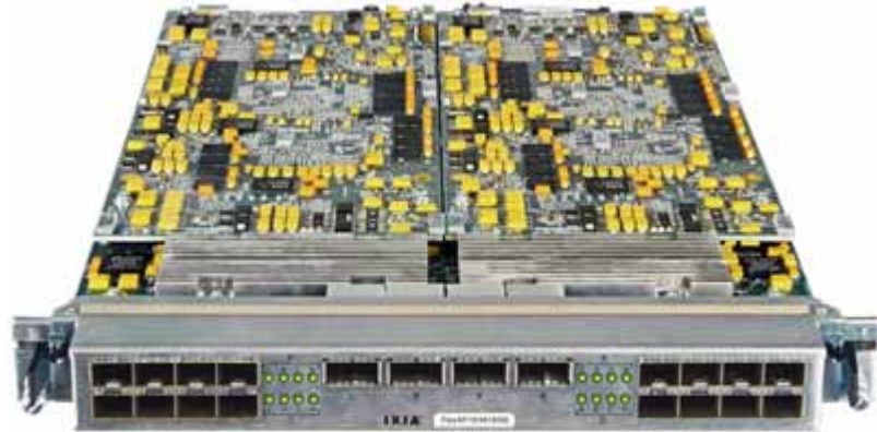
Figure 33-4. Xcellon-Flex Module-FlexFE40QP
