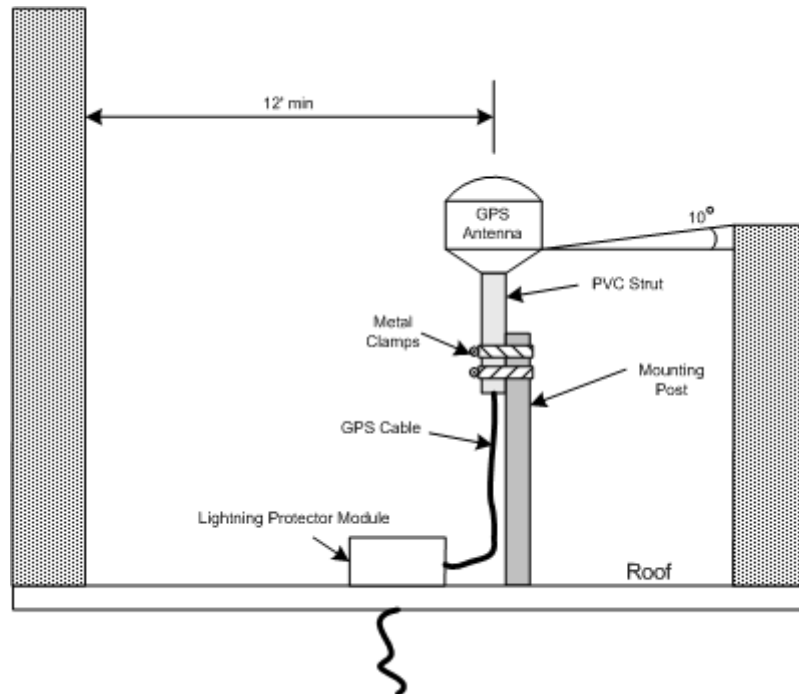
Figure C-1. GPS Installation Requirements
