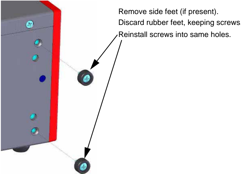
Figure 5-2. Remove Side Feet (If Present)
