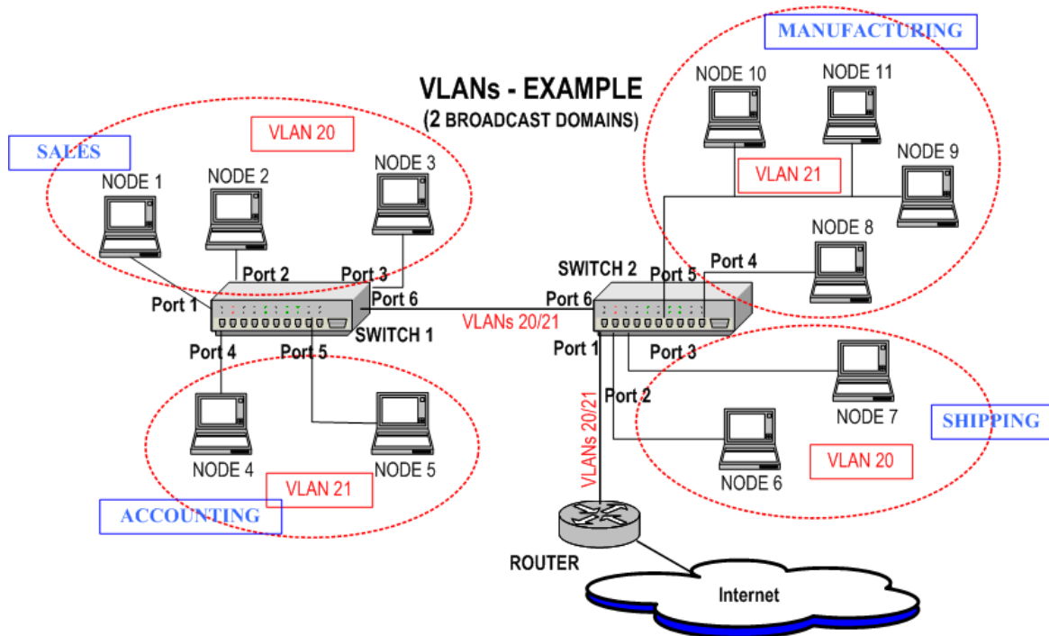
Figure 2-41. Example of VLANs
