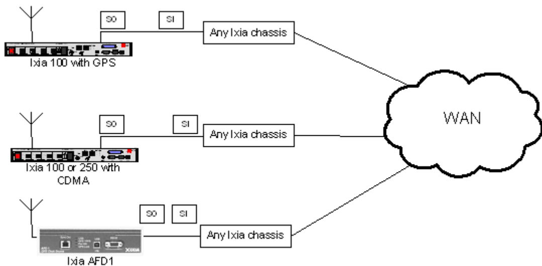
Figure 2-4. Virtual Chaining
