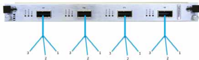
Figure 34-7. 3x10GE Multis CXP mode
