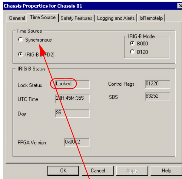
Figure 19-3. Chassis Properties AFD2 - Time Source
