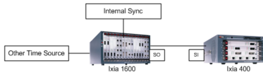
Figure 2-3. Physical Chaining
