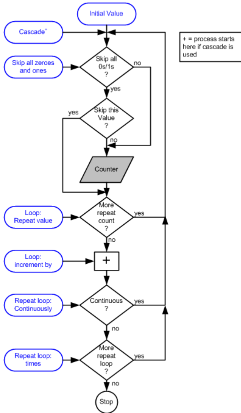
Figure 2-48. UDF IPv4 Mode Operation
