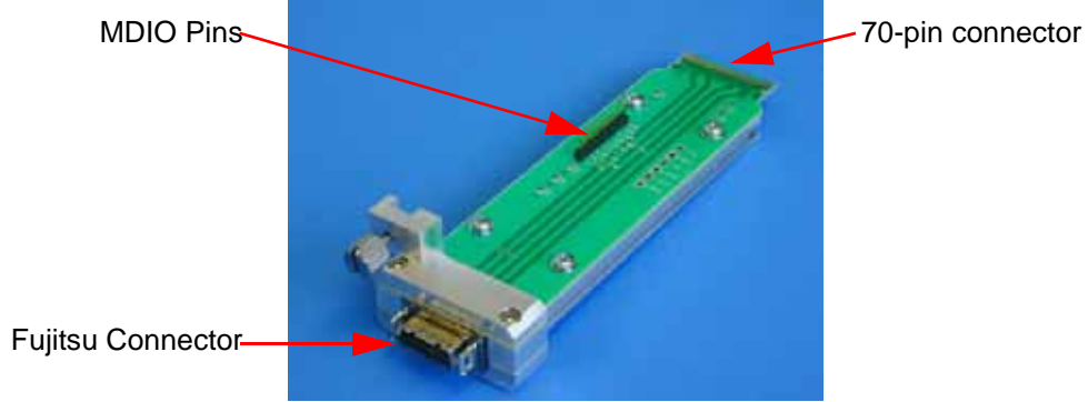
Figure A-9. CX4 and XAUI MDIO Pinouts
