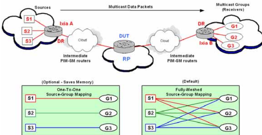
Figure 3-16. PIM-SM Source-Group Mapping Example
